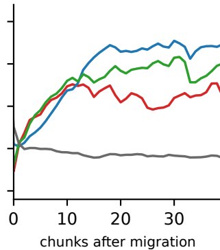
bird, k=2
