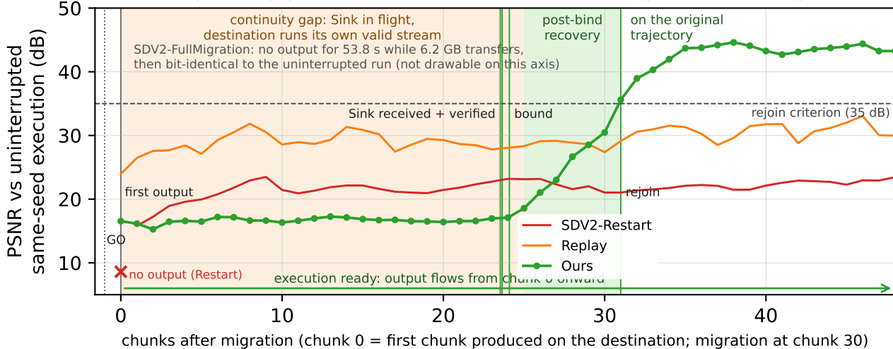
(a) Continuity after a physical handoff elves-01 → elves-02 (1000 Mbps, seed 0, k=2, rep 2)
