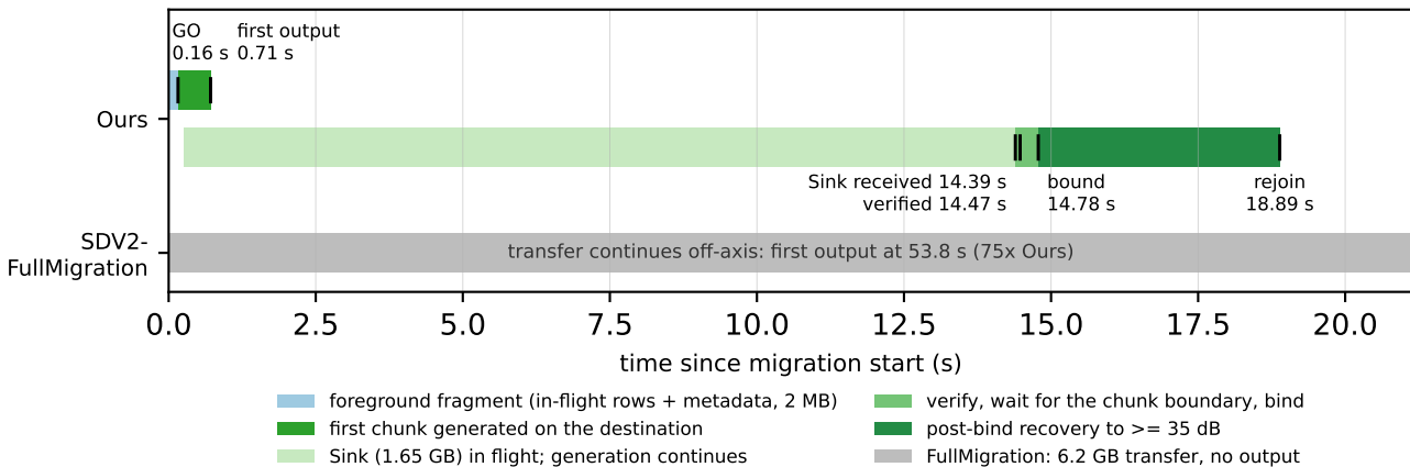
(b) Latency decomposition for Ours (1000 Mbps): execution handoff vs continuity handoff
