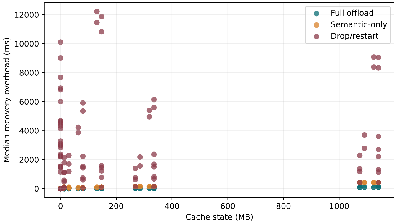
Cache size versus recovery cost
