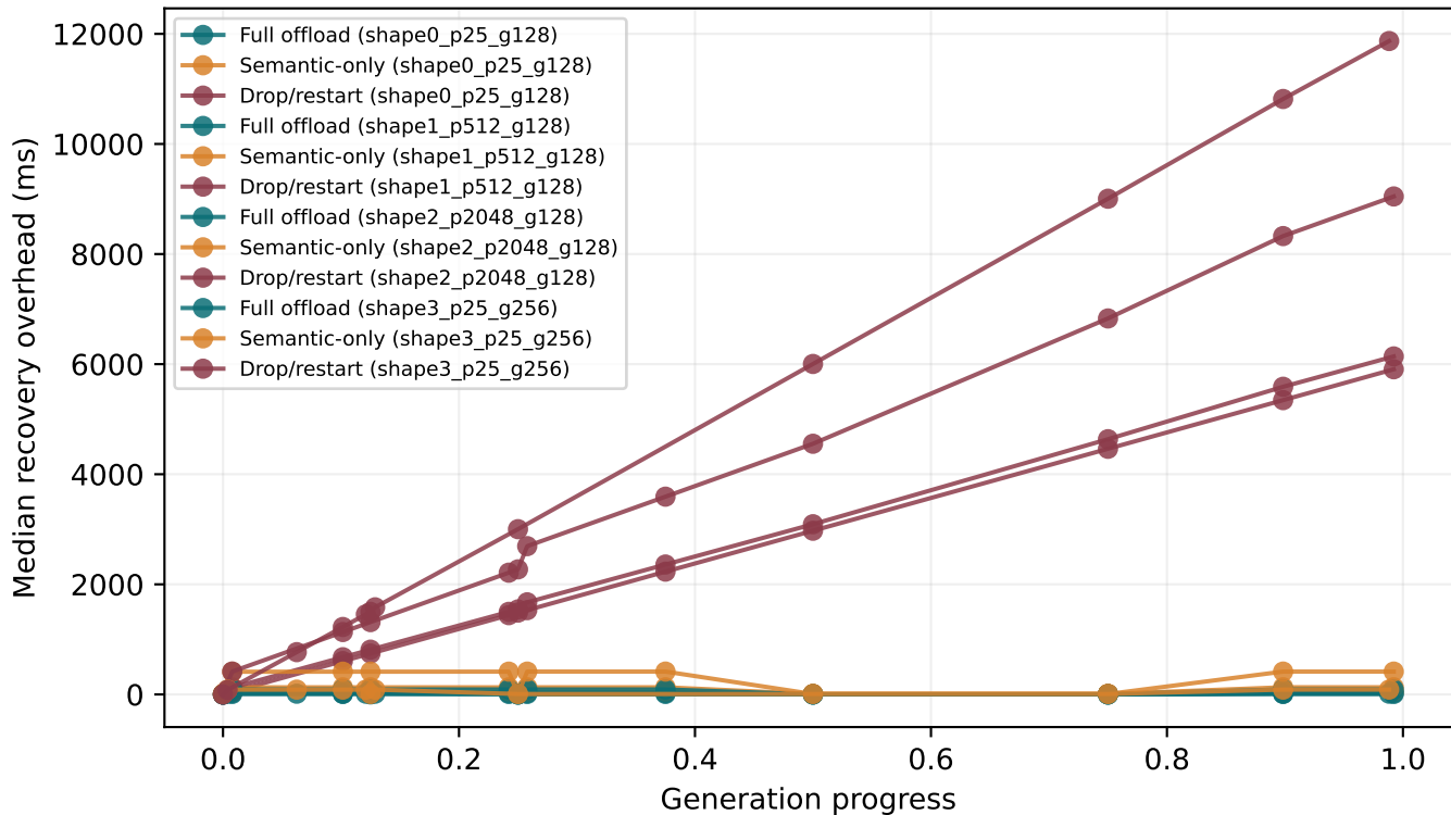
Dual cache recovery cost
