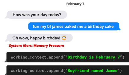
Figure 1. MemGPT (left) writes data to persistent memory after it receives a system alert about limited context space.
