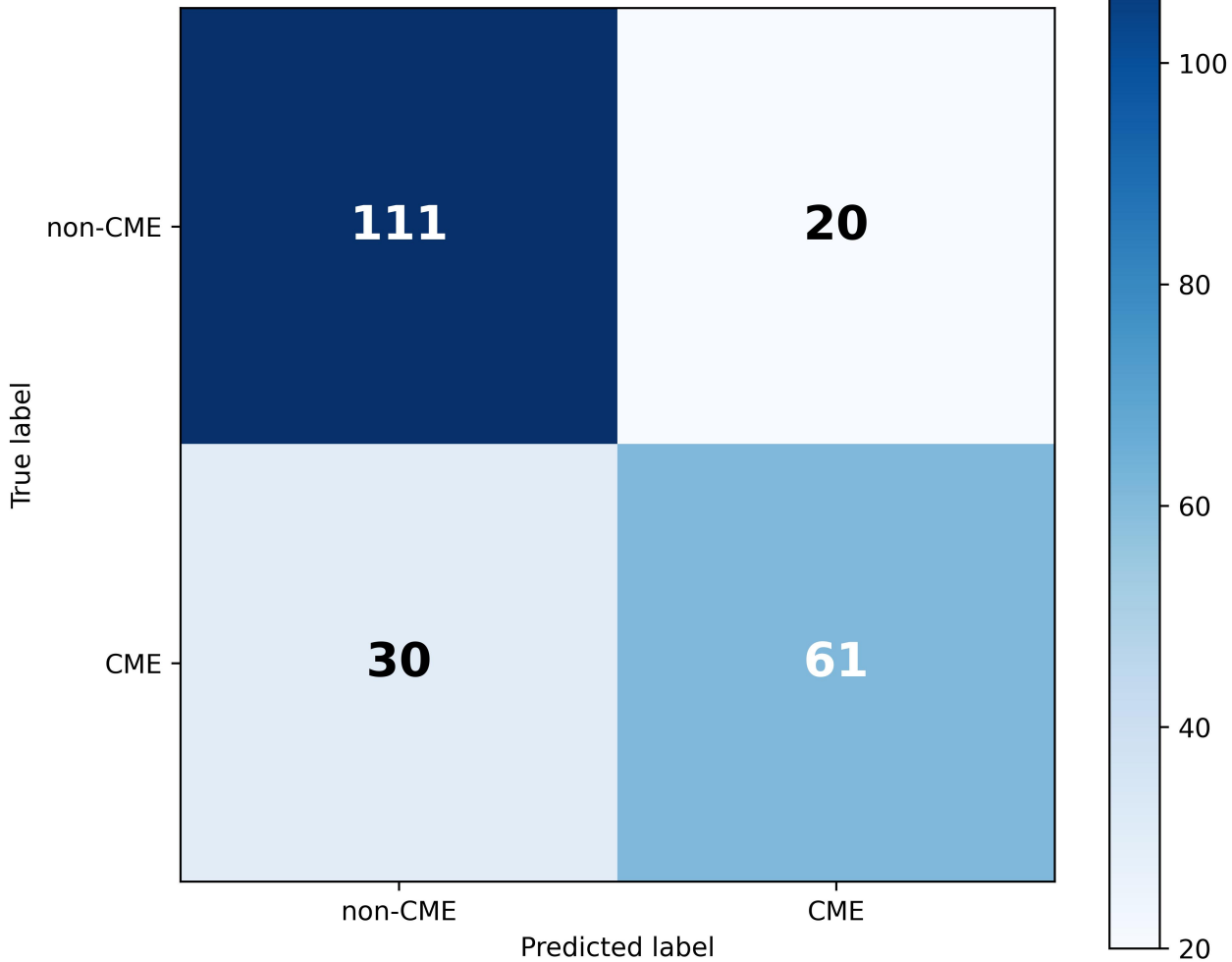
Confusion Matrix (threshold = 0.5)
