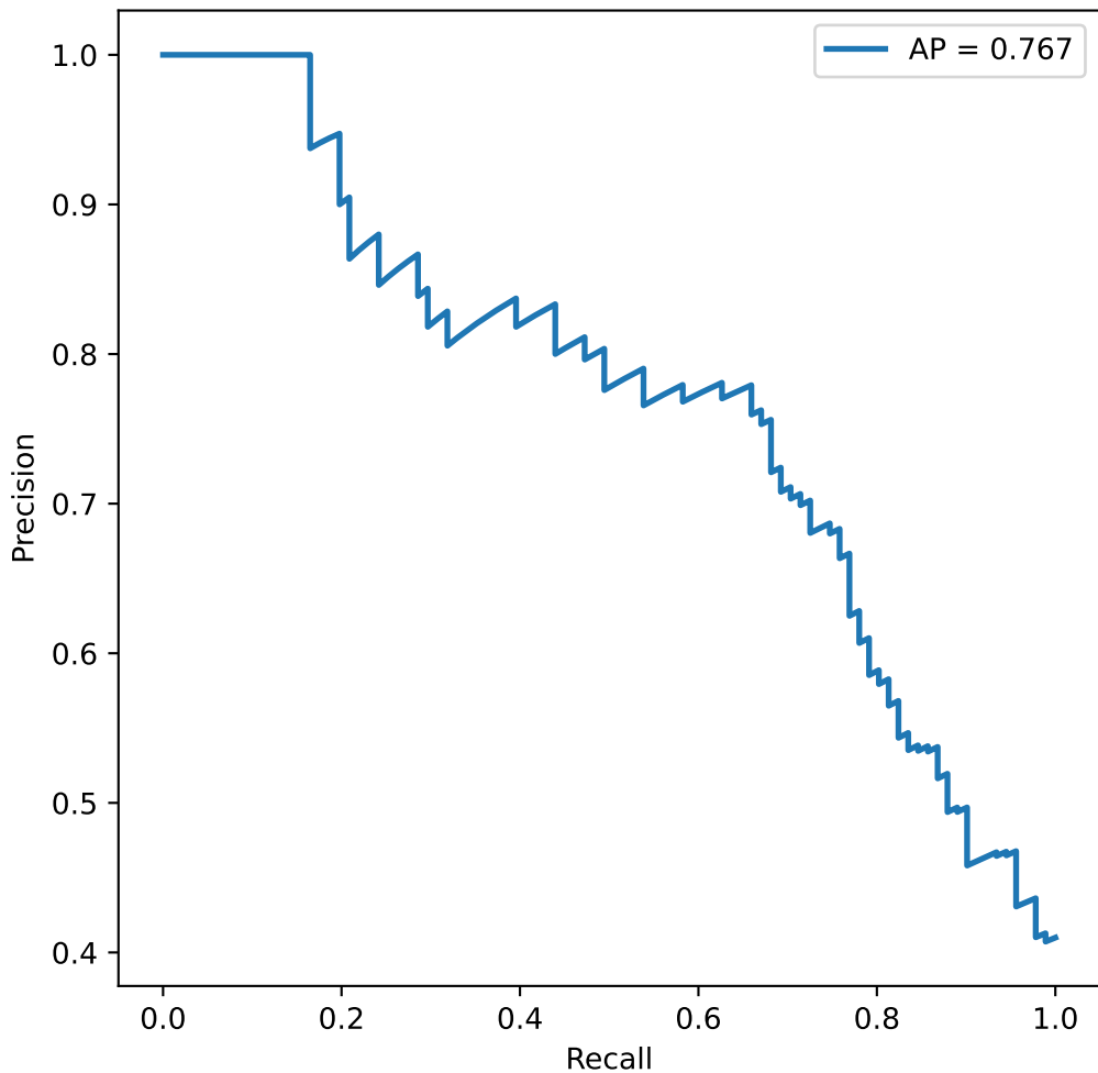
5-Fold Cross-Validated PR Curve
