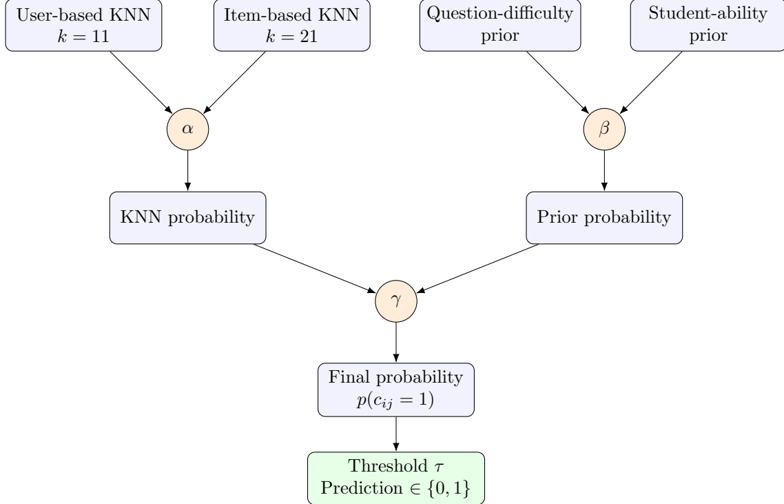
Figure 4: Schematic of the Part B hybrid predictor. User- and item-based KNN outputs are blended by \alpha ; the question-difficulty and student-ability priors are blended by \beta ; the resulting KNN and prior probabilities are blended by \gamma and thresholded at \tau to produce the final prediction.
