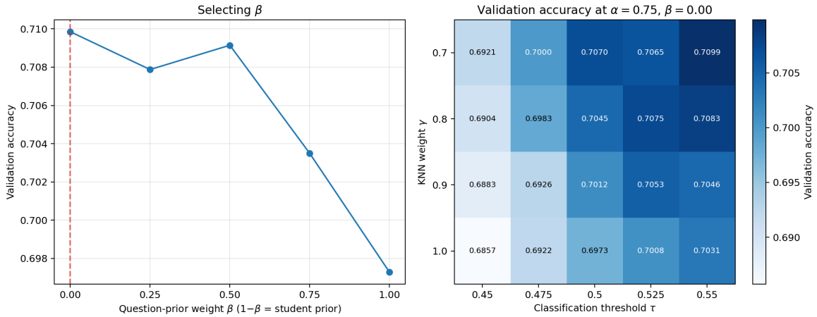
Figure 6: Validation accuracy as a function of the prior-blend weight \beta (left), and as a function of the KNN-vs-prior weight \gamma and threshold \tau at the selected \alpha, \beta (right).
