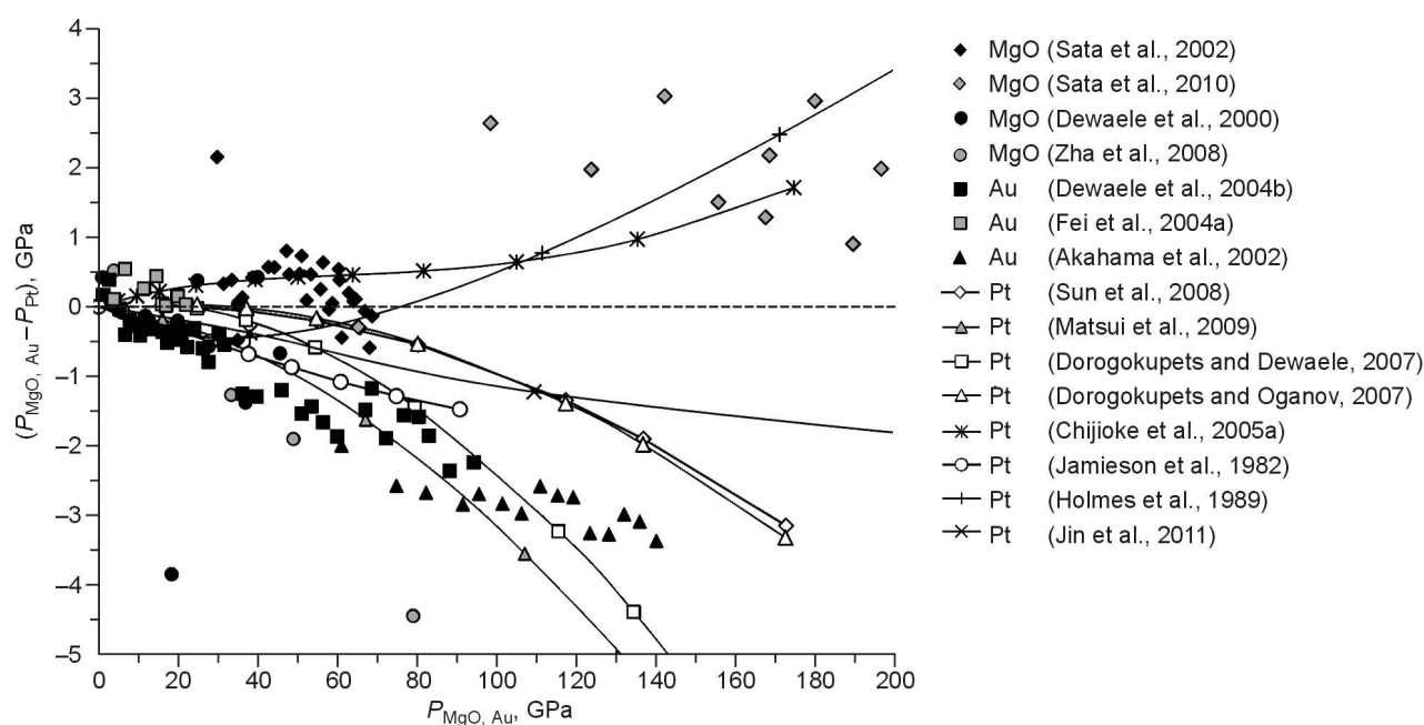
Fig. 8. Difference in pressure between our EOSs for MgO and Au and the EOS for Pt, calculated from the results of simultaneous measurements of the MgO–Pt and Au–Pt cell parameters on the room-temperature isotherm borrowed from literature. Also, the difference between the EOSs for Pt from (Chijioke et al., 2005a; Dorogokupets and Dewaele, 2007; Dorogokupets and Oganov, 2007; Holmes et al., 1989; Jamieson et al., 1982; Jin et al., 2011) and our EOS for Pt is shown.
