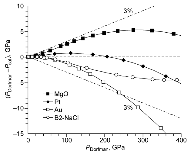
Fig. 12. Difference between the pressures calculated by the pressure scales from Dorfman et al. (2012) and the pressures calculated by the EOSs for MgO, Pt, Au, and B2-NaCl from Table 4.
