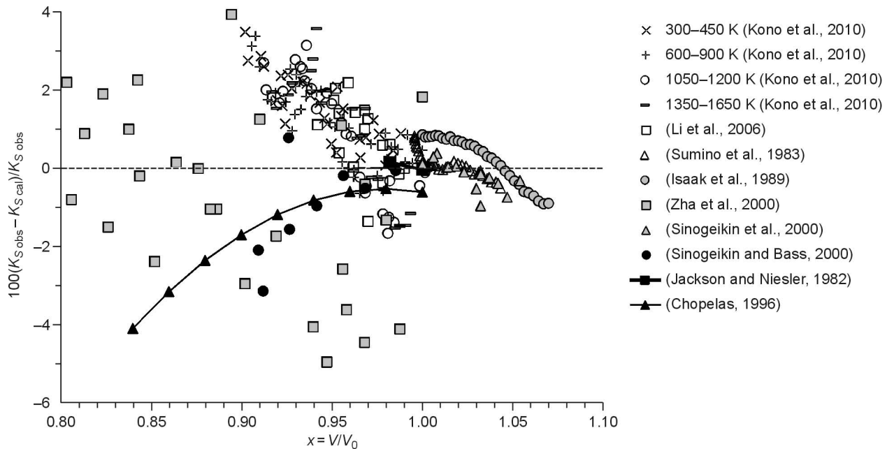
Fig. 5. Difference (in %) between the measured ( K_{S \text{ obs}} ) (Kono et al., 2010) and calculated ( K_{S \text{ cal}} ) (by our EOS (Table 4)) adiabatic bulk moduli of MgO. Measurements in other mentioned works were performed on the room-temperature isotherm.
