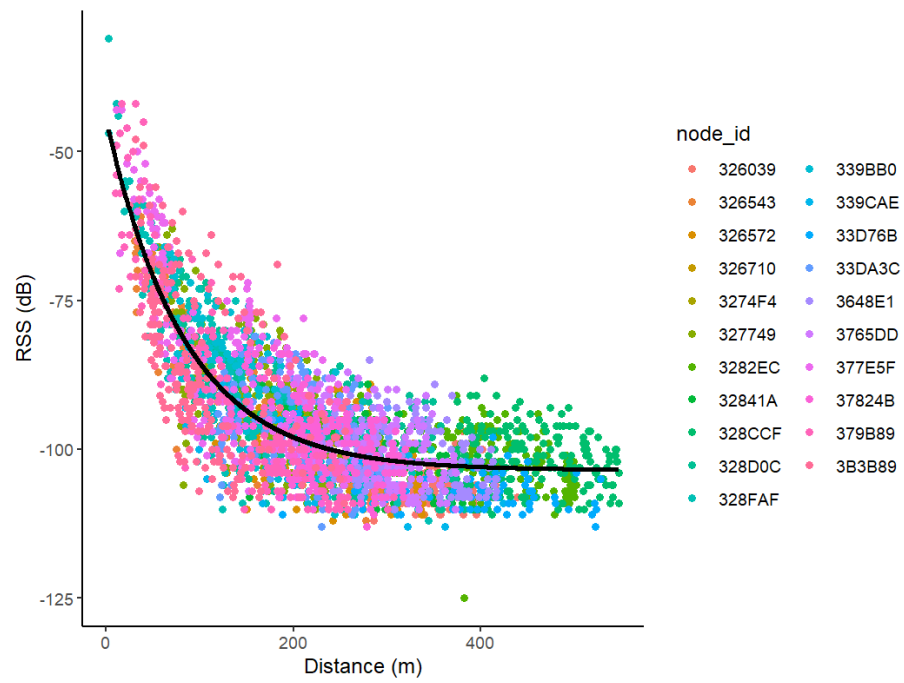
Figure 10.1: RSS vs. Distance with Predicted Line
