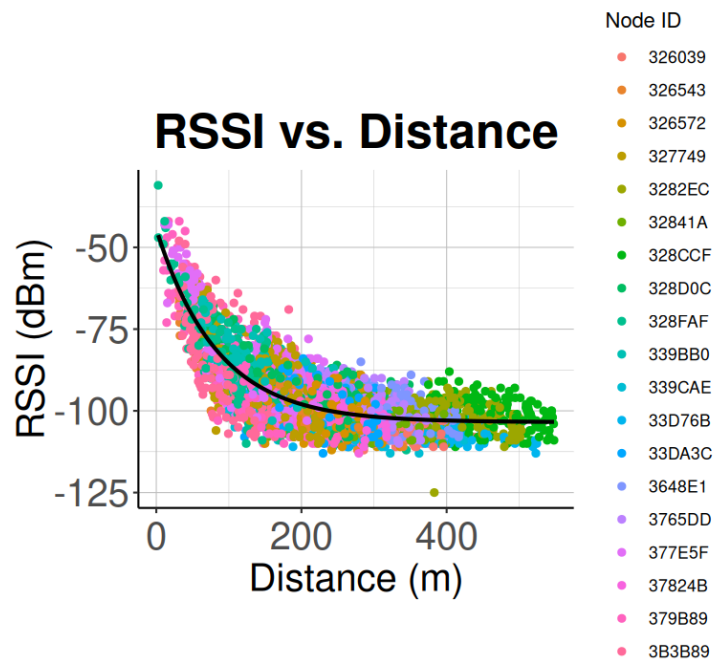
Figure 5.5: RSSI vs. Distance
