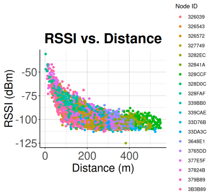
Figure 5.4: RSSI vs. Distance
