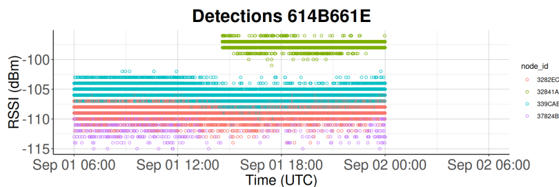
Figure 7.1: Scatter plot of RSSI vs time by Node
