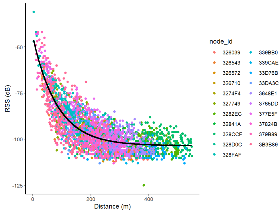
Figure 11.1: RSS vs. Distance with Predicted Line
