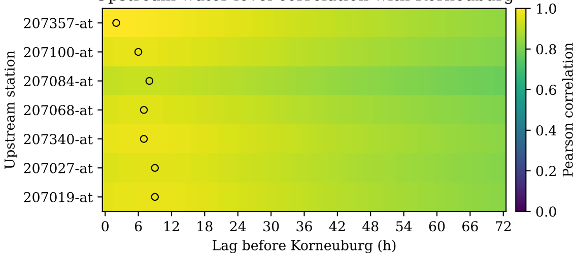
Upstream water level correlation with Korneuburg
