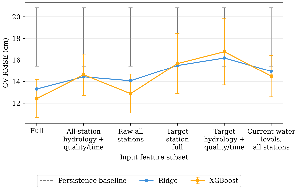
Cross-validation RMSE by feature subset and model
