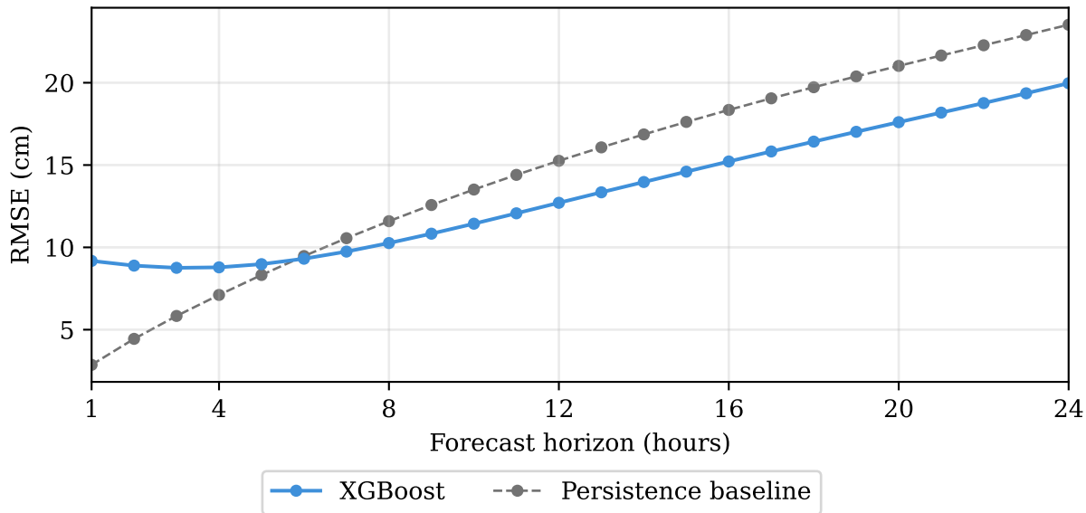
Test set RMSE by forecast horizon (XGBoost)
