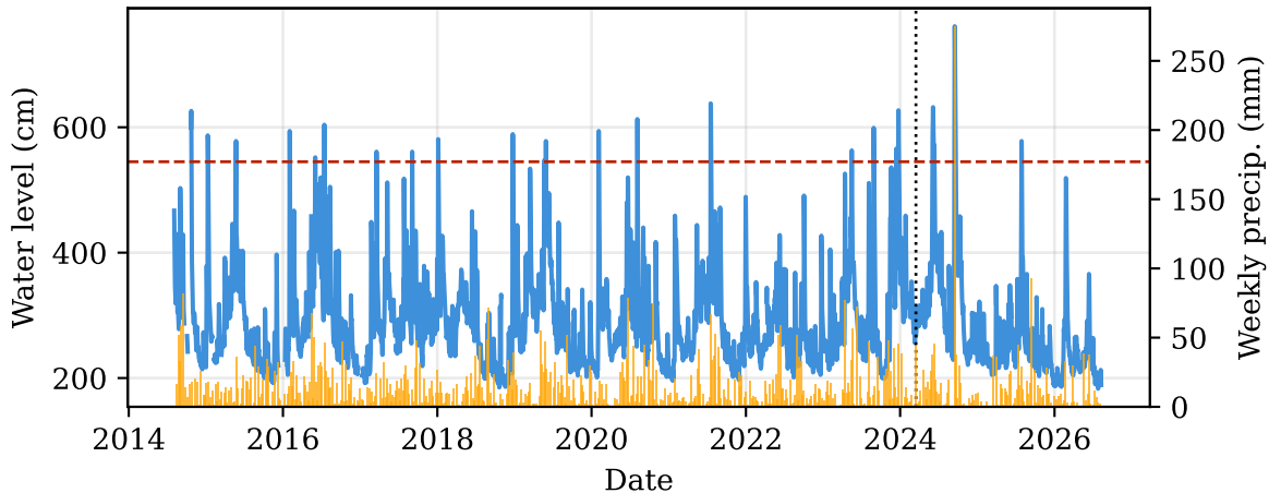
Korneuburg water level (207241-at)
