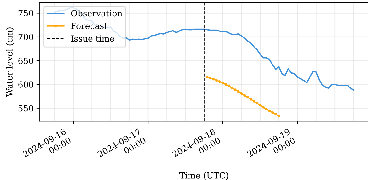
Bad XGBoost forecast (RMSE: 109.61)
