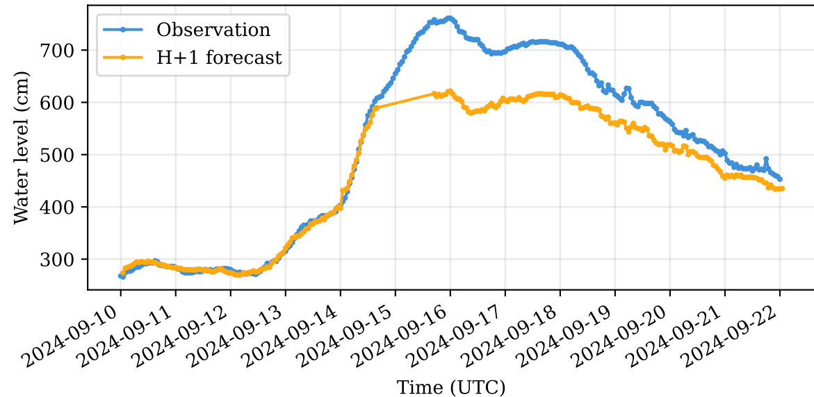
XGBoost H+1 forecast against observed water level
