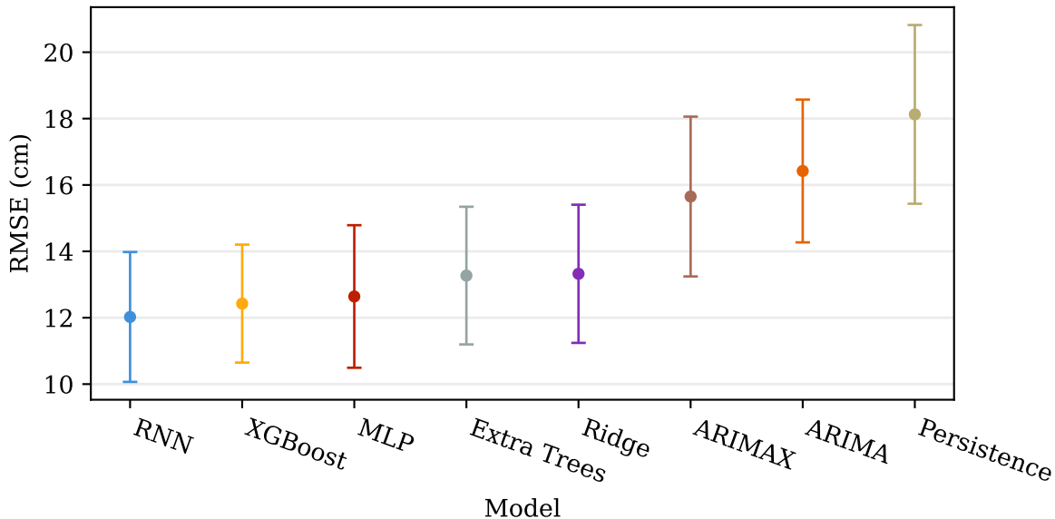
Aggregate Cross-Validation RMSE (mean \pm standard deviation)
