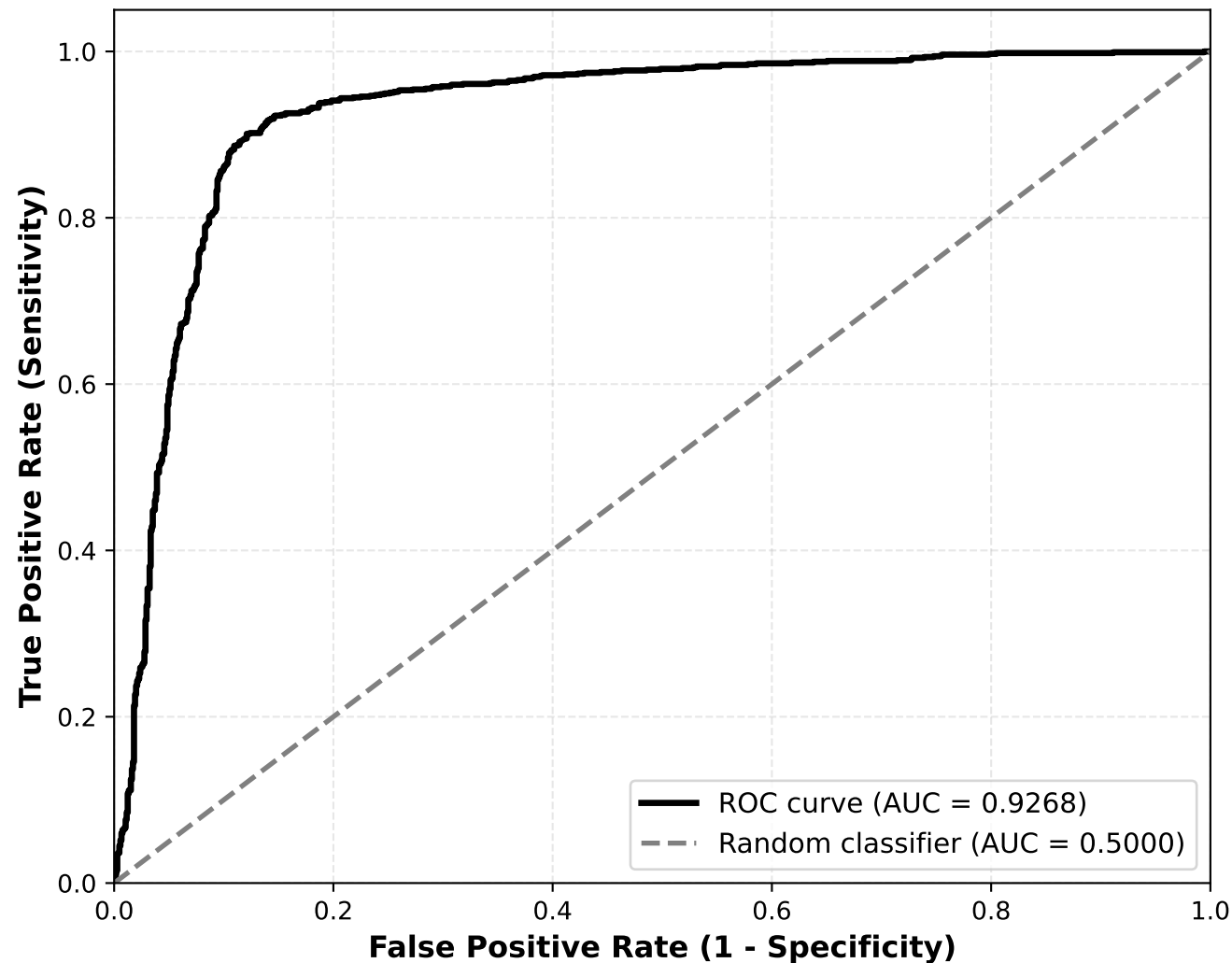
ROC Curve - EfficientNet-B0 + SVC
