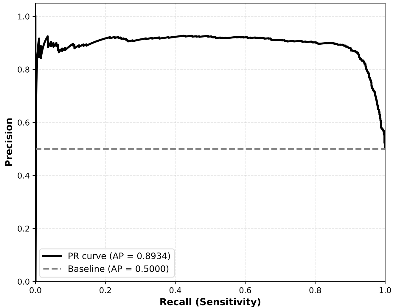
Precision-Recall Curve - EfficientNet-B0 + SVC
