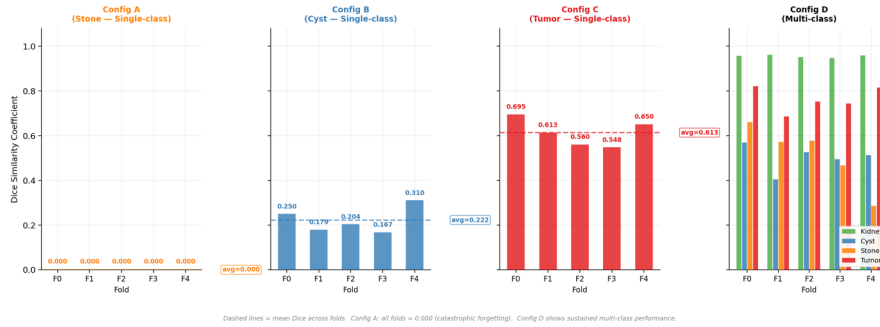
Figure 17. Per-fold Dice across all configurations
