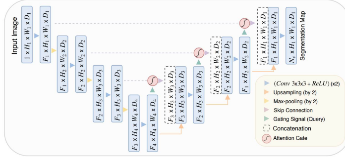
Figure 4. Attention Mechanism. Reprinted from [43].
