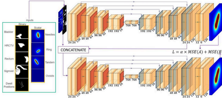
Figure 7. 3D Cascade Architecture. Retrieved from [57].
