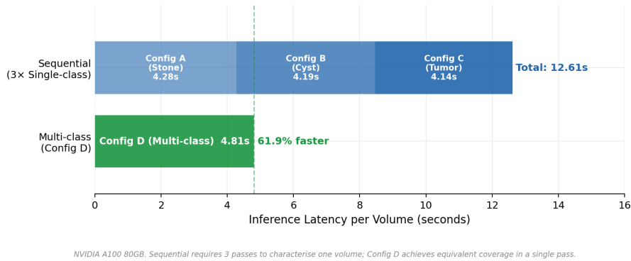
Figure 22. Inference Latency Comparison
