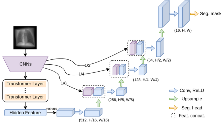
Figure 5. Hybrid Transformers. Reprinted from [46].
