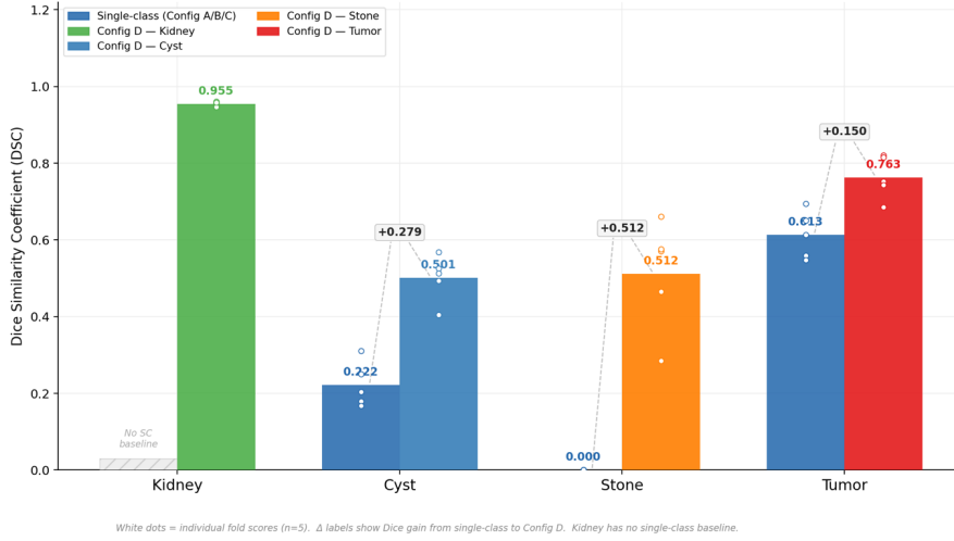
Figure 20. Single-Class vs Multi-Class Dice Comparison
