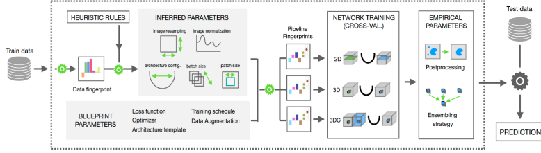
Figure 6. nnU-Net Configuration Hierarchy. Reprinted from [53]
