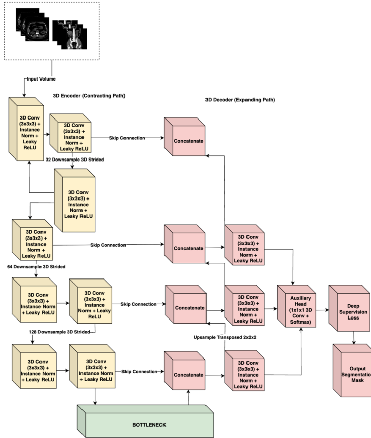
Figure 11. nnU-Net V2 Architecture
