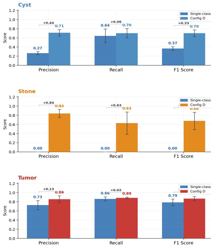
Figure 24. Precision, Recall, F1 Single-class VS Multi-class
