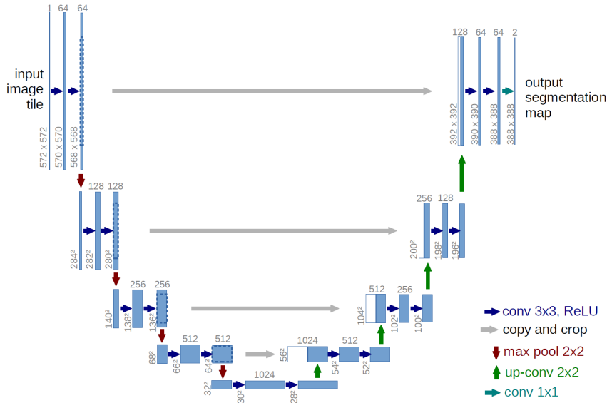
Figure 1. The U-Net Architecture. Illustration of the contracting and expanding paths with skip connections. Reprinted from [12].
