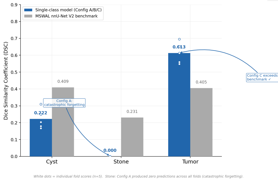
Figure 16. Single-class vs MSWAL Benchmark
