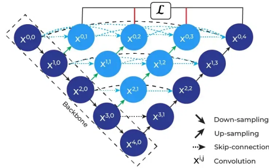
Figure 3. U-Net++ Architecture. Reprinted from [42].
