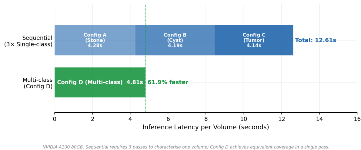
Figure 22. Inference Latency Comparison
