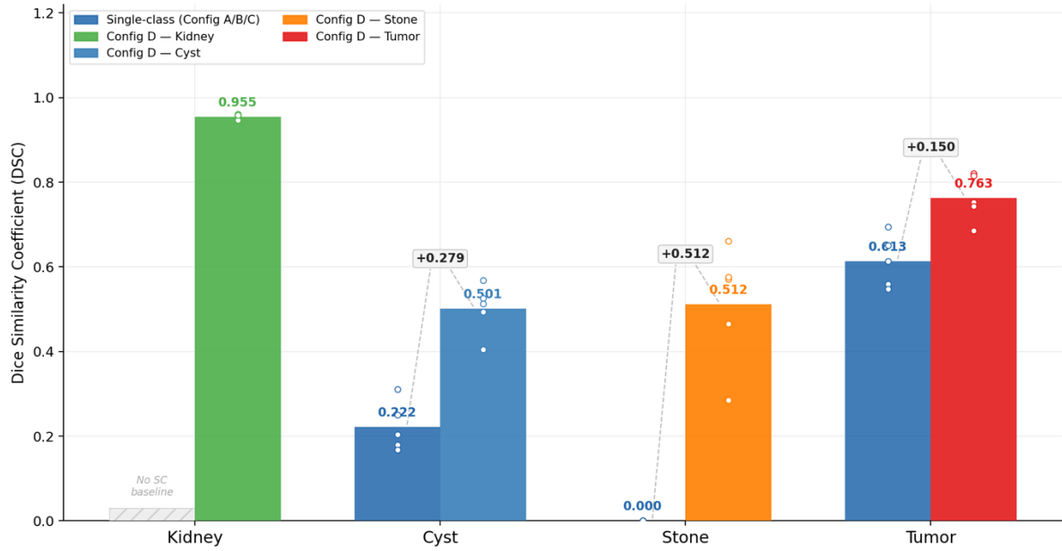
Figure 20. Single-Class vs Multi-Class Dice Comparison
