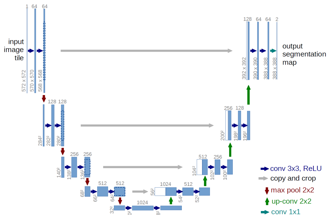
Figure 5. The U-Net Architecture. Illustration of the contracting and expanding paths with skip connections. Reprinted from [12].
