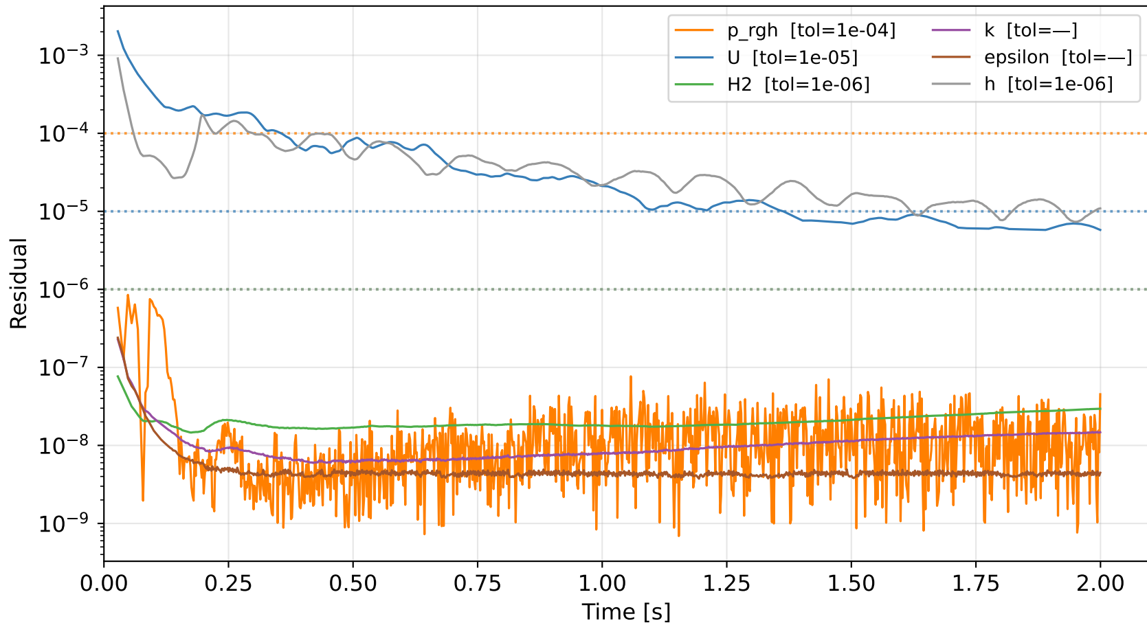
Bunkering_07 — Solver residuals (dotted lines = PIMPLE residualControl tolerance)
