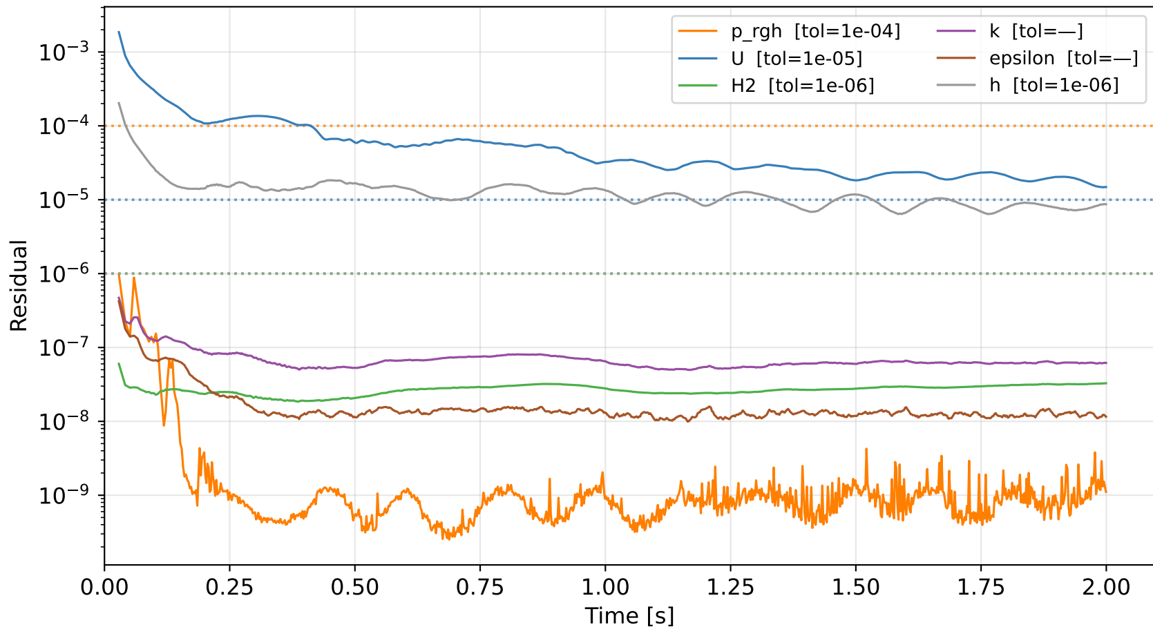
Bunkering_09 — Solver residuals (dotted lines = PIMPLE residualControl tolerance)
