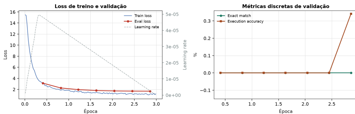
Figure 7: Fine-tuning completo com oncomx + gradient checkpointing – curvas de treino.
