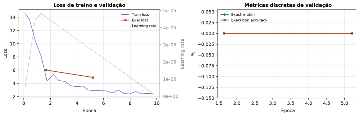
Figure 5: Fine-tuning few-shot – curvas de treino.
