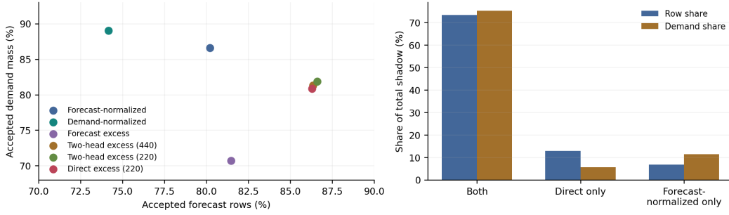
Figure 1: Strong forecaster. Left: three-seed means under the same row-coverage threshold selection; row and demand coverage disagree. Right: first-seed direct-excess versus forecast-normalized-error acceptance sets. The extra direct-only set contains more rows but less demand than the relative-only set. Both panels describe the consumed development shadow.
