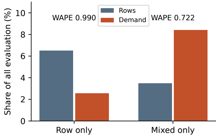
The stronger predictor still reallocates
