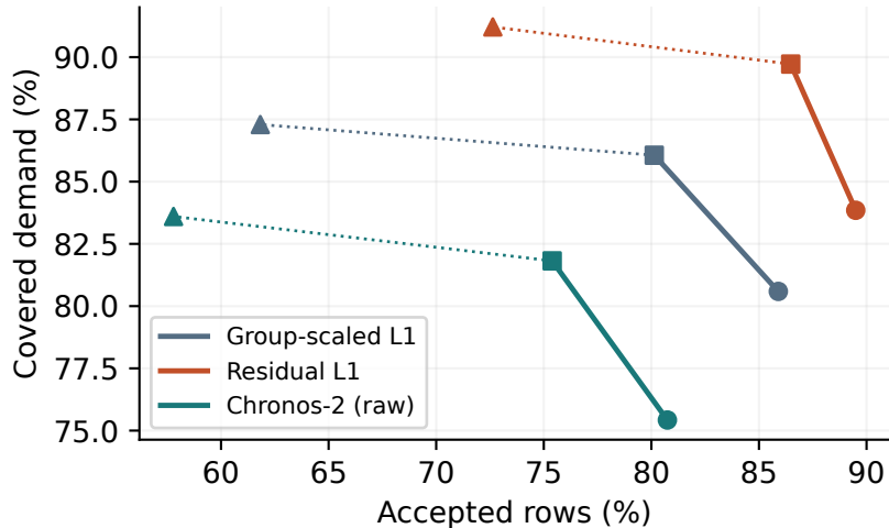
Accuracy improves both coverages
