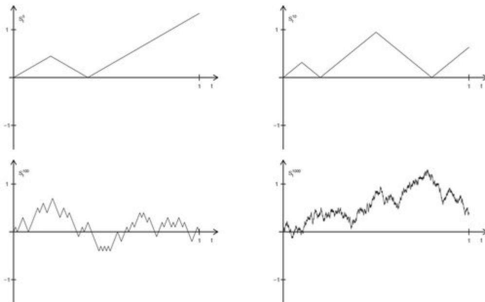
Fig. 3.4. The first few approximation steps in Donsker's construction: n = 5, 10, 100 and 1000 .
