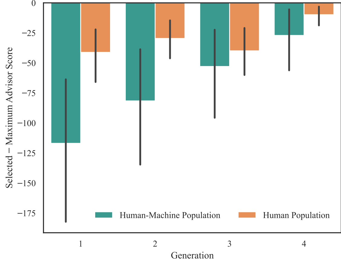
Regret of Advisor Selection
