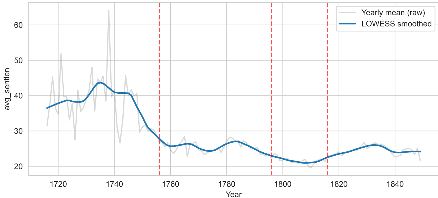
International: avg_sentlen with detected breakpoints
