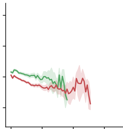
Qwen2.5-1.5B-Instruct
