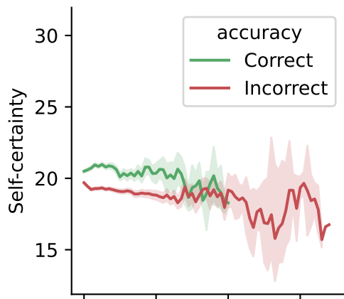
Qwen2.5-0.5B-Instruct
