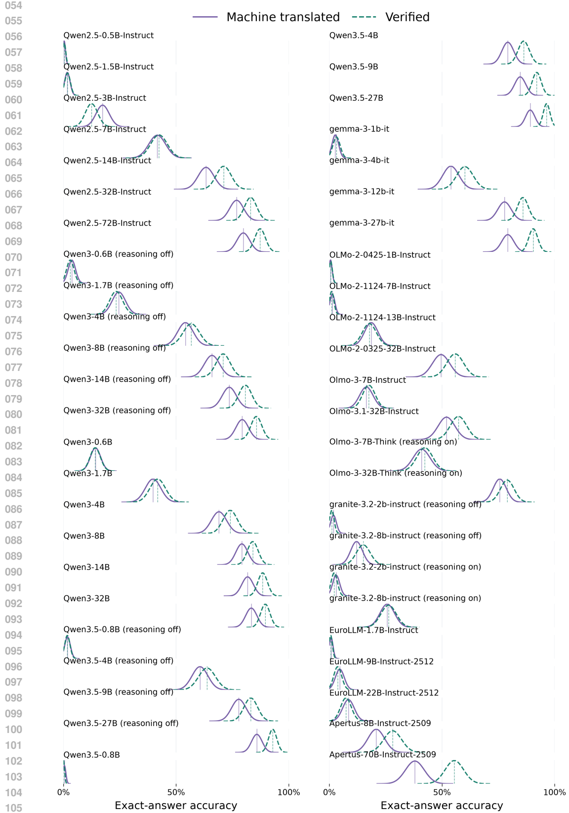
Figure 2: Distribution of model performances on the machine-translated and verified Icelandic subsets.
