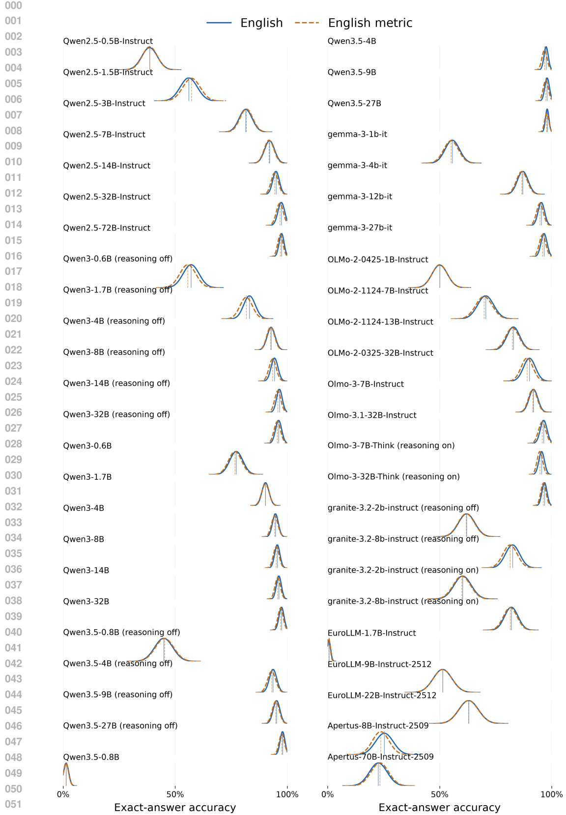
Figure 1: Distribution of model performances on the English and metric-converted English subsets.
