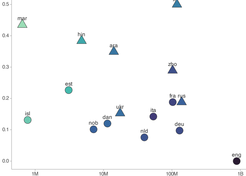
Typological distance
