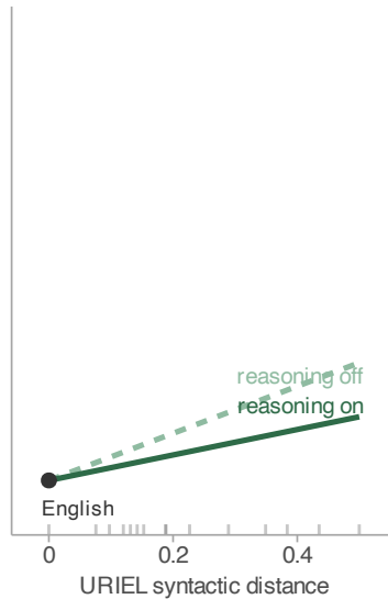
Reasoning × distance
