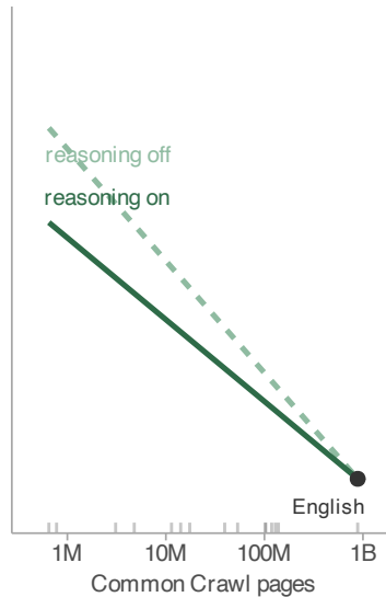
Reasoning × resource
