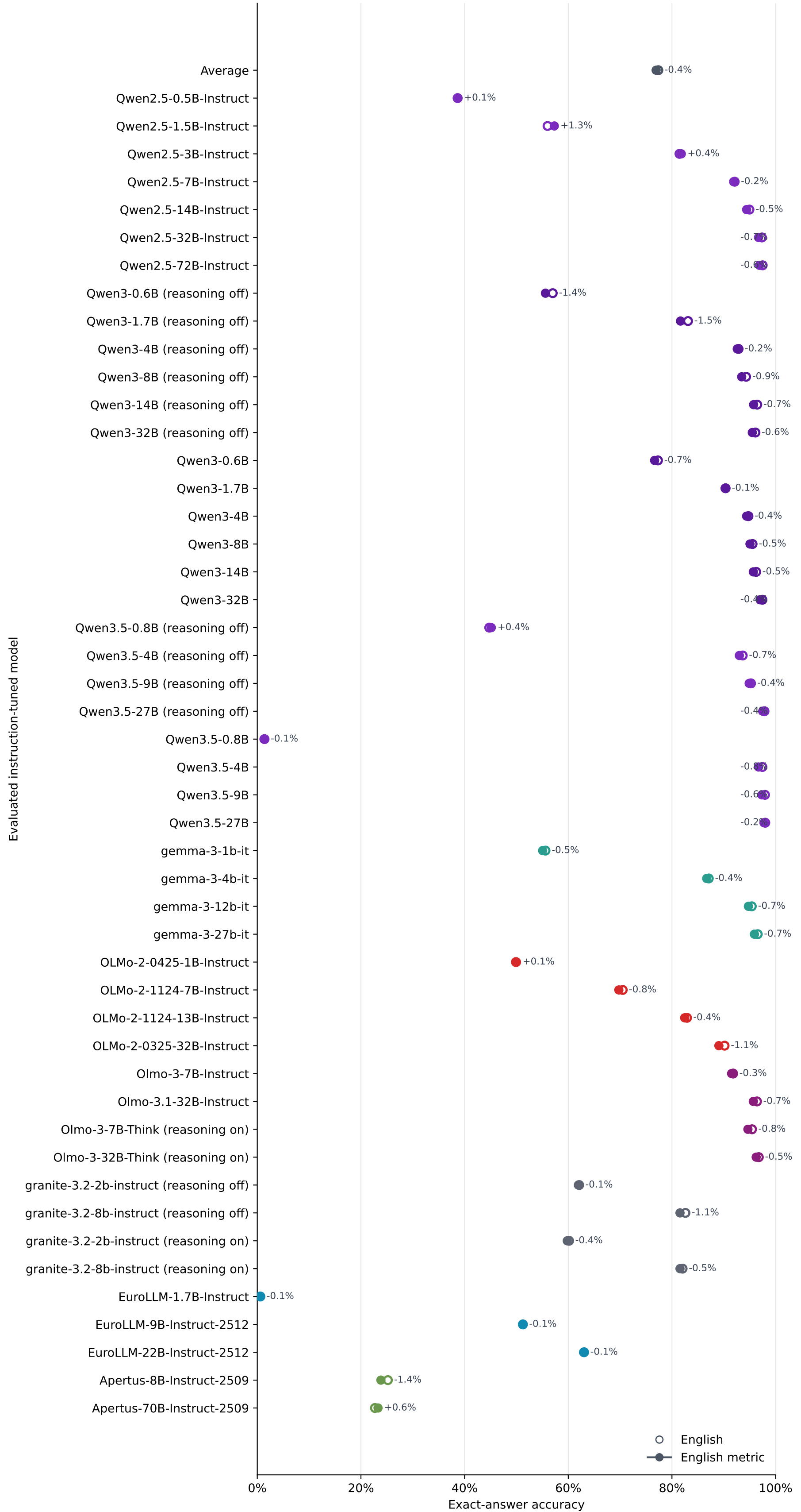
English metric vs English accuracy (Synthetic numerical variants)
