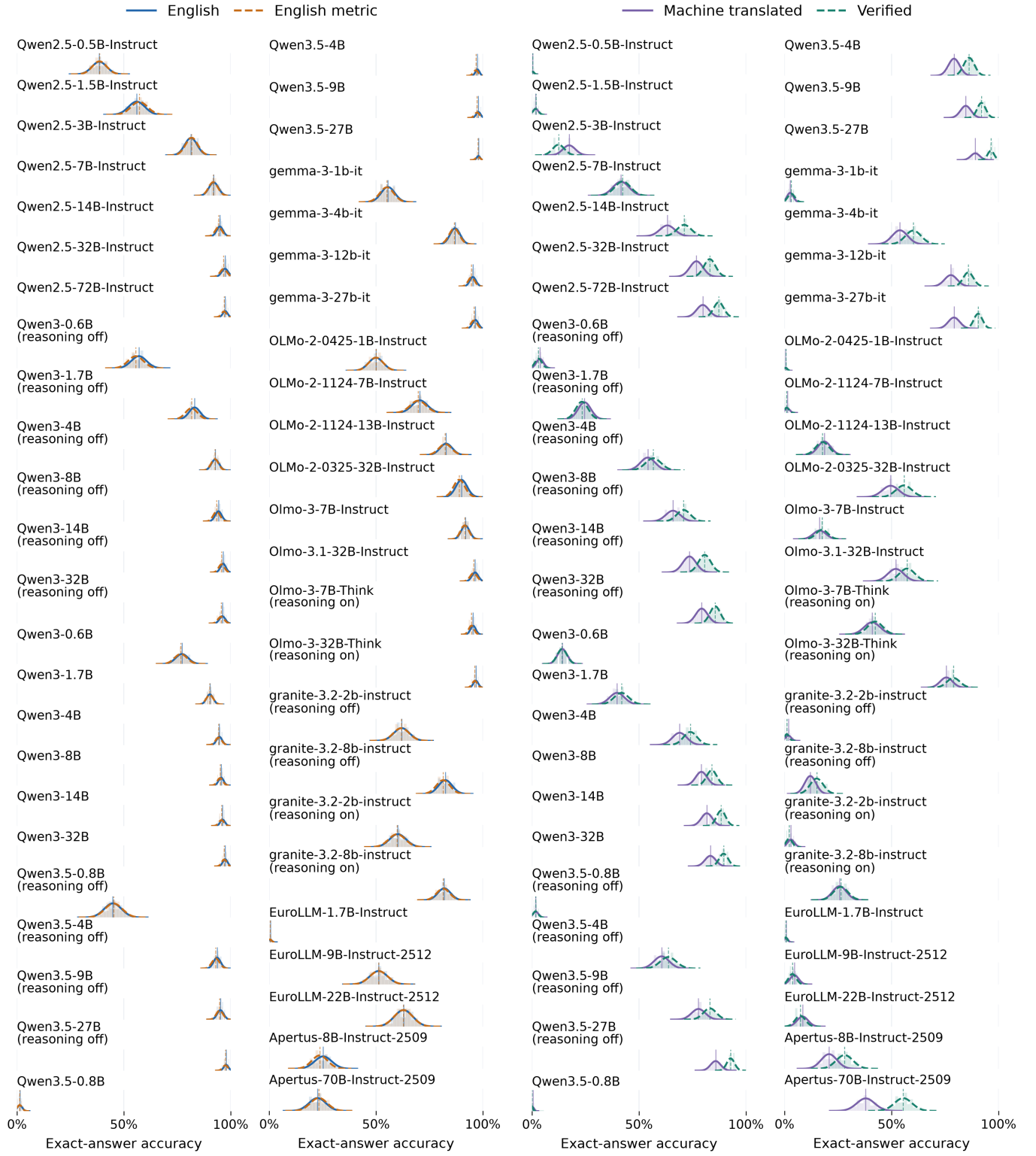
Figure 1: Distribution of model performances on the English and metric-converted English subsets.
