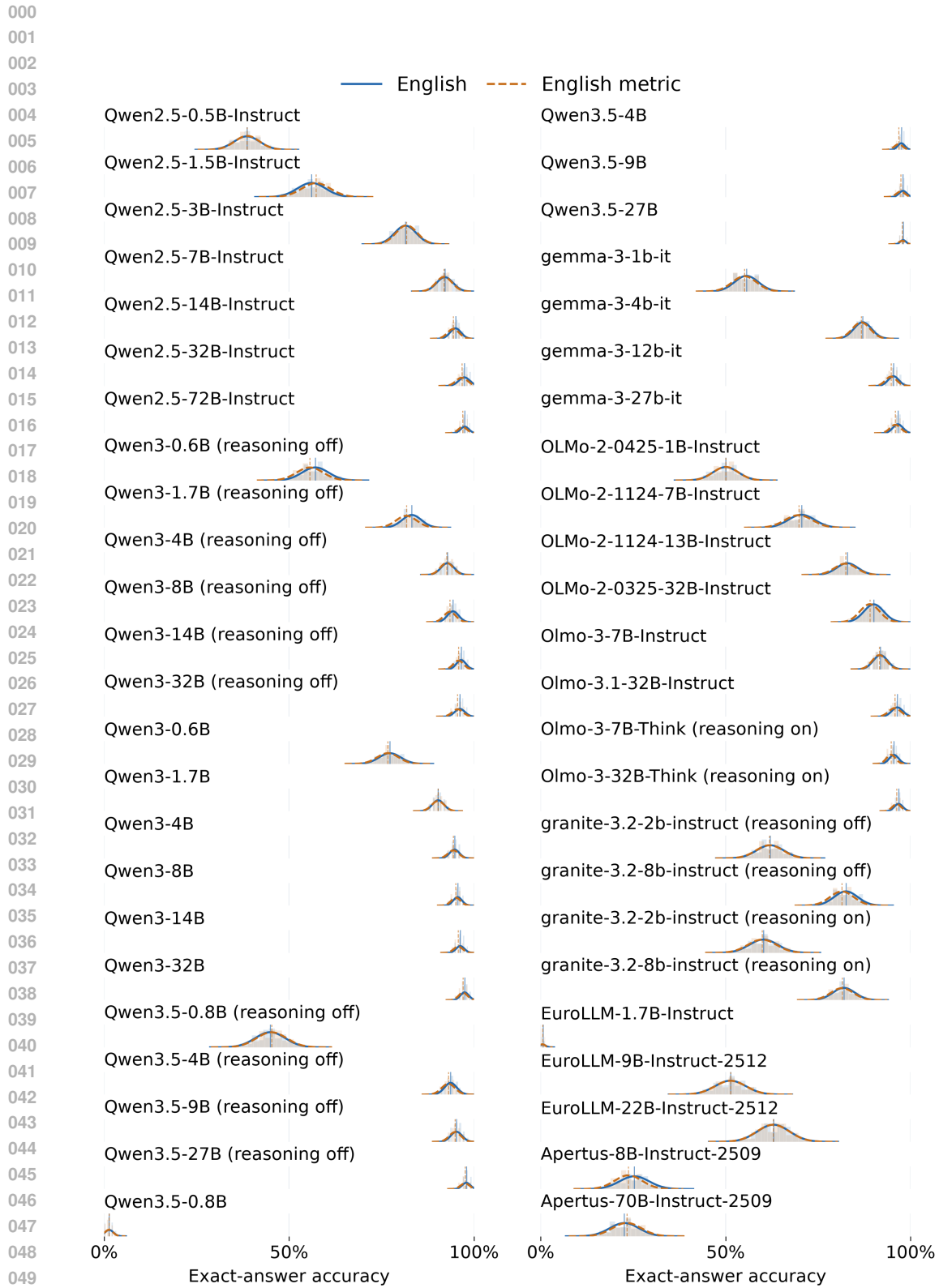
Figure 1: Distribution of model performances on the English and metric-converted English subsets.
