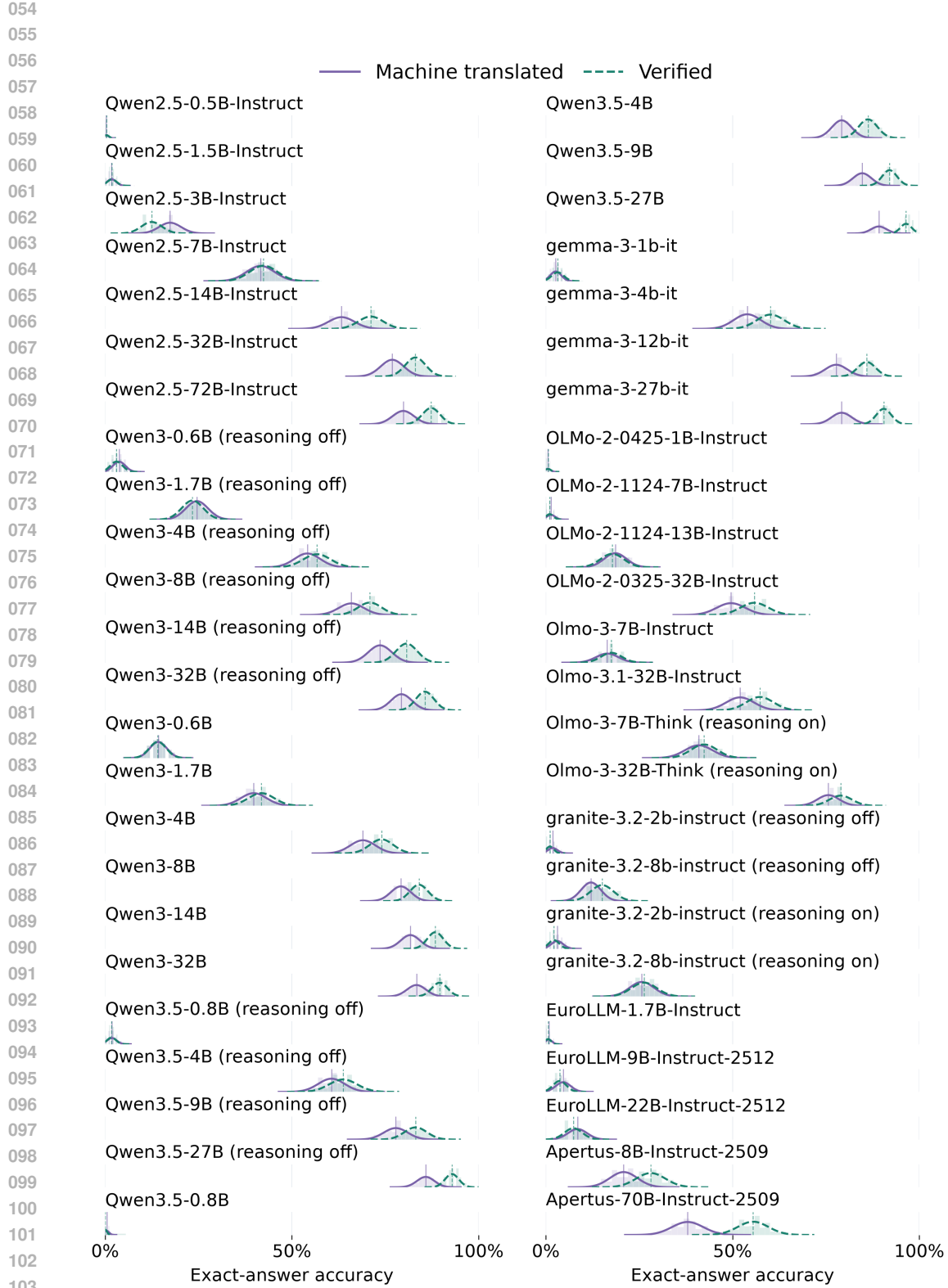
Figure 2: Distribution of model performances on the machine-translated and verified Icelandic subsets.
