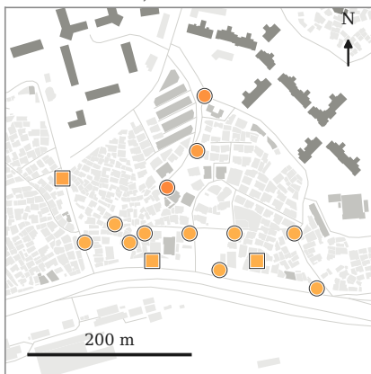
(a) LCZ 1 Compact high-rise
