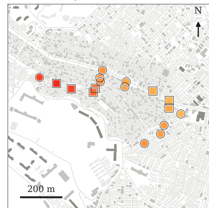
(c) LCZ 3 Compact low-rise
