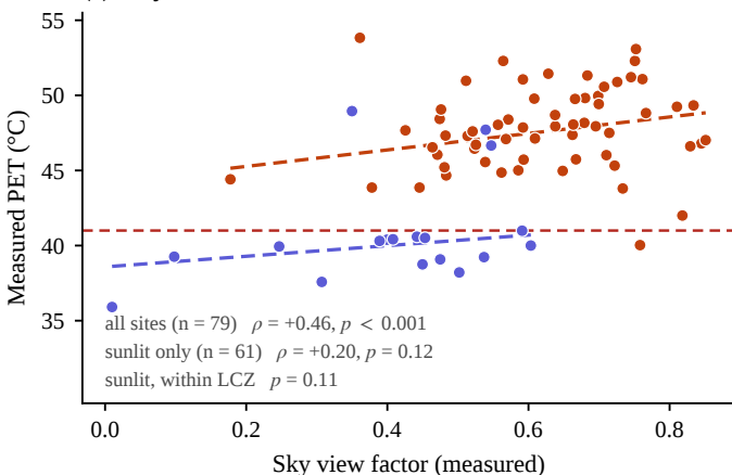
(c) Sky view factor vs PET
