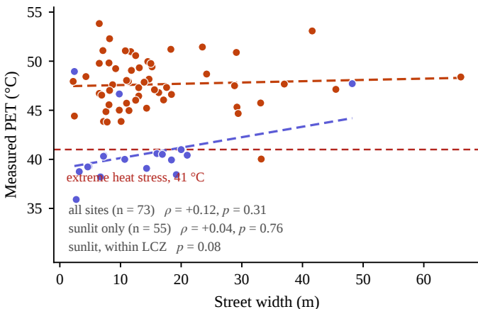
(a) Street width vs PET
