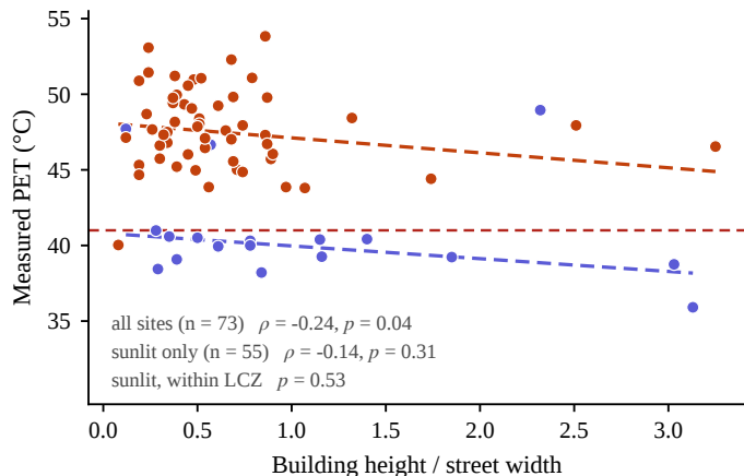
(b) Height-to-width ratio vs PET
