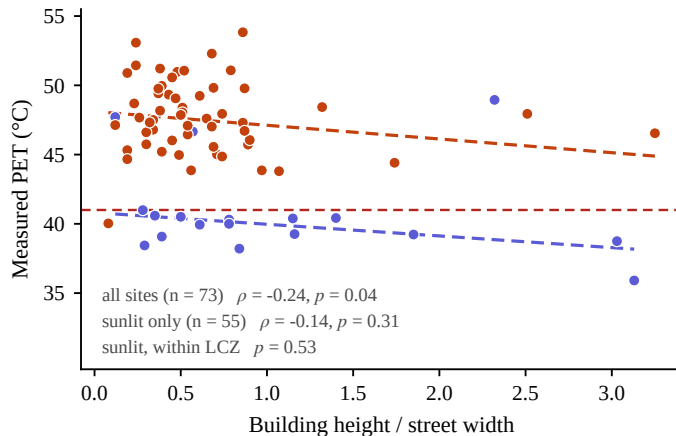
(b) Height-to-width ratio vs PET
