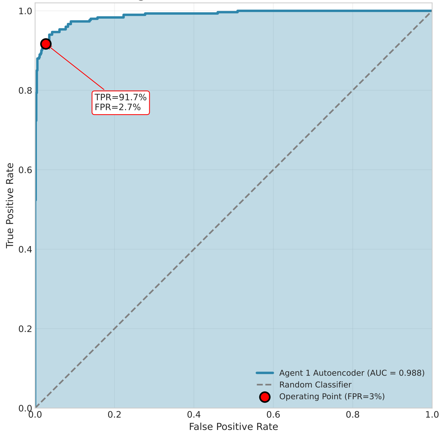
Agent 1: Autoencoder ROC Curve
