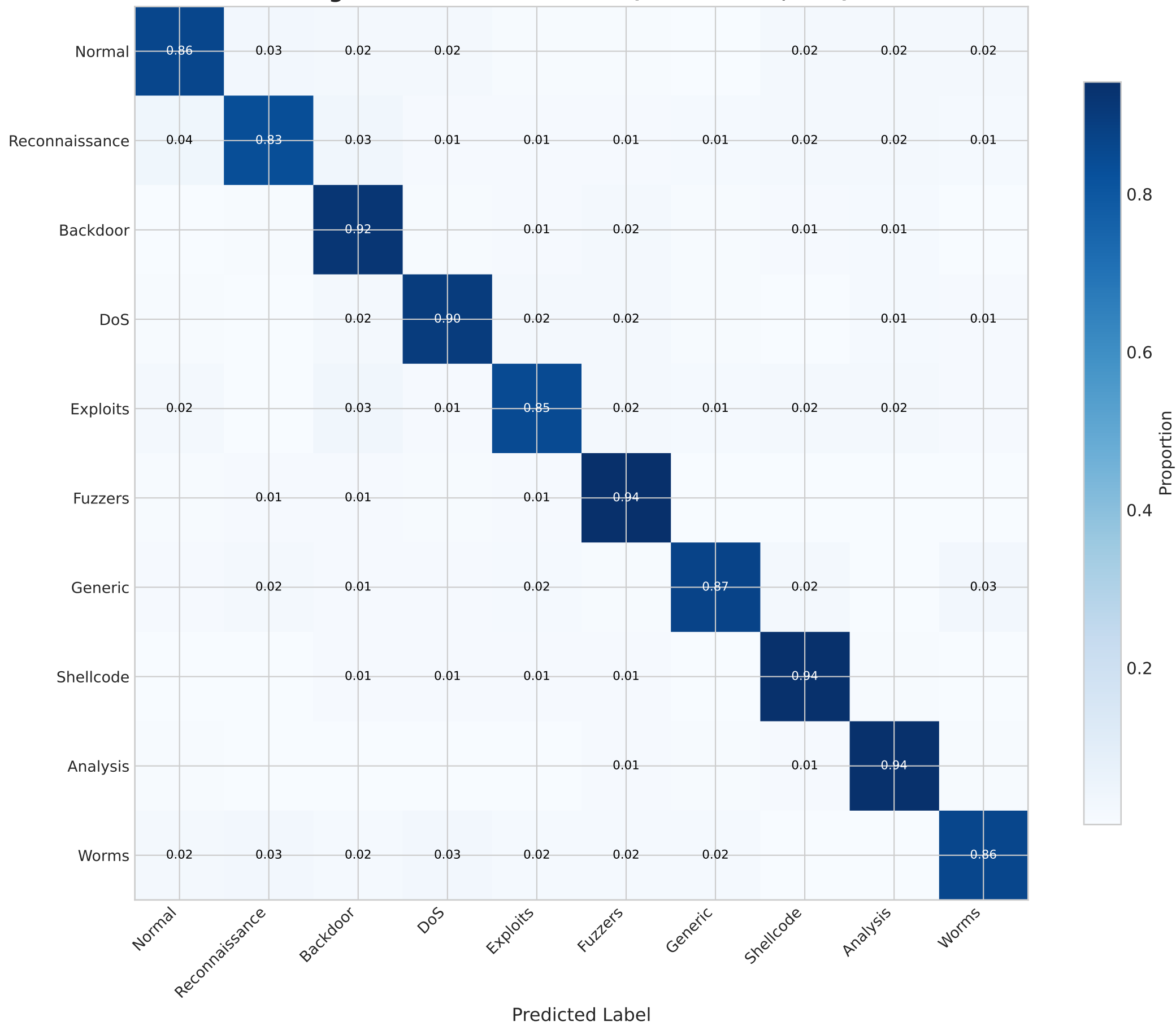
Agent 2: Confusion Matrix (DP-XGBoost, \epsilon=4 )
