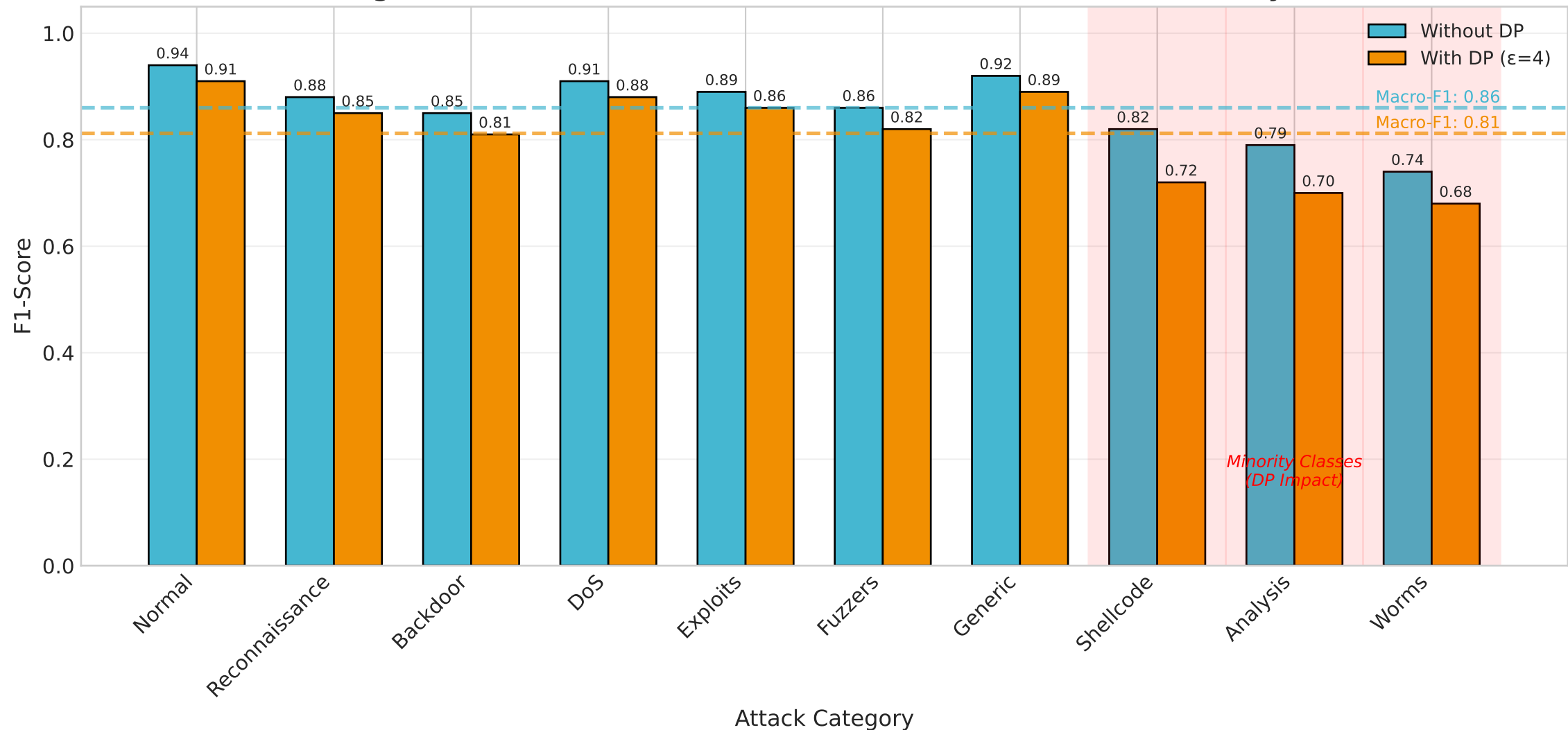
Agent 2: Per-Class F1-Scores (XGBoost with Differential Privacy)
