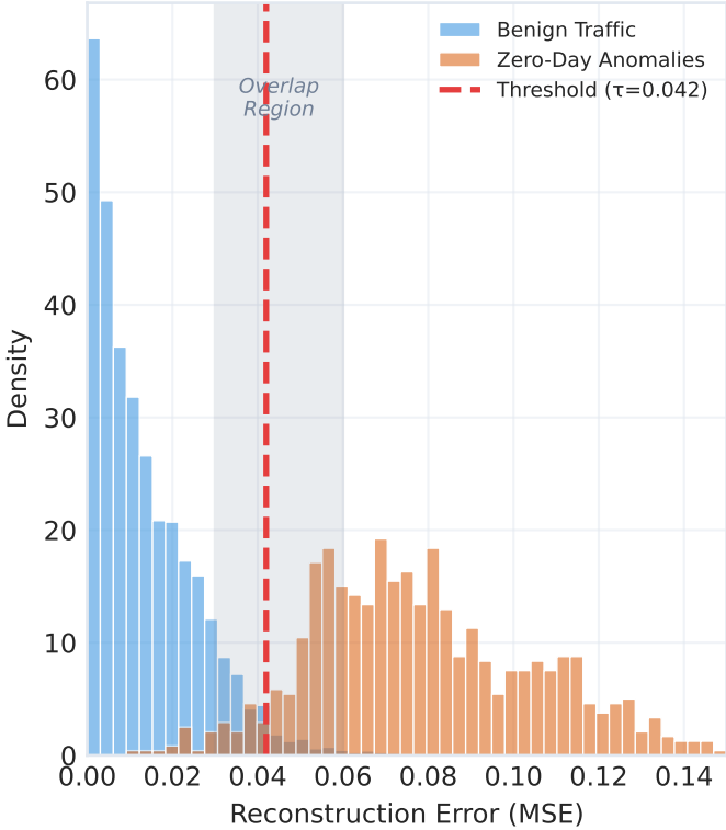
Autoencoder Reconstruction Error Distribution
