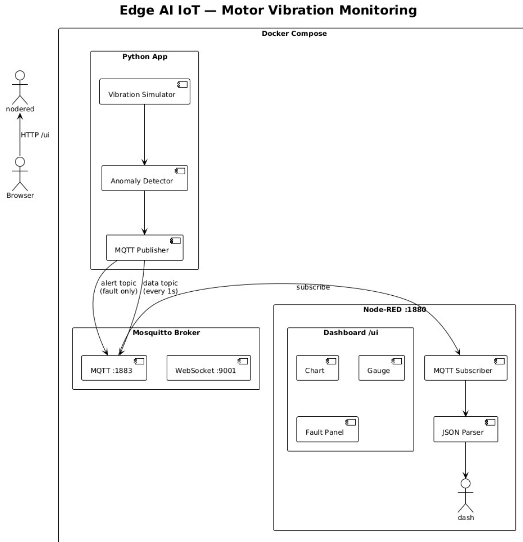
Figure 2: System Architecture Data Flow
