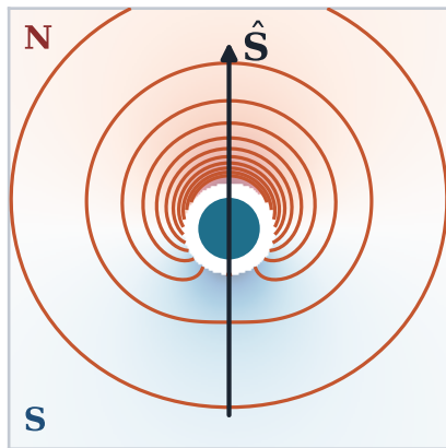
(b) ASTG: +(s_g/r)\lambda_1 \cos \theta
