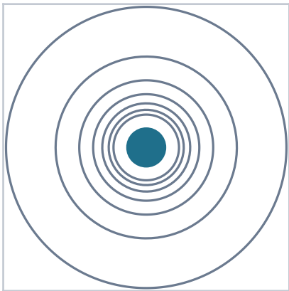
(a) Newtonian: \Phi = -GM/r
