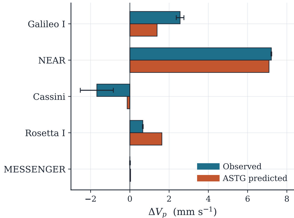
Single global \lambda_1 , all geometry-driven
