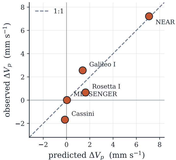
NEAR: 1.8\% error
