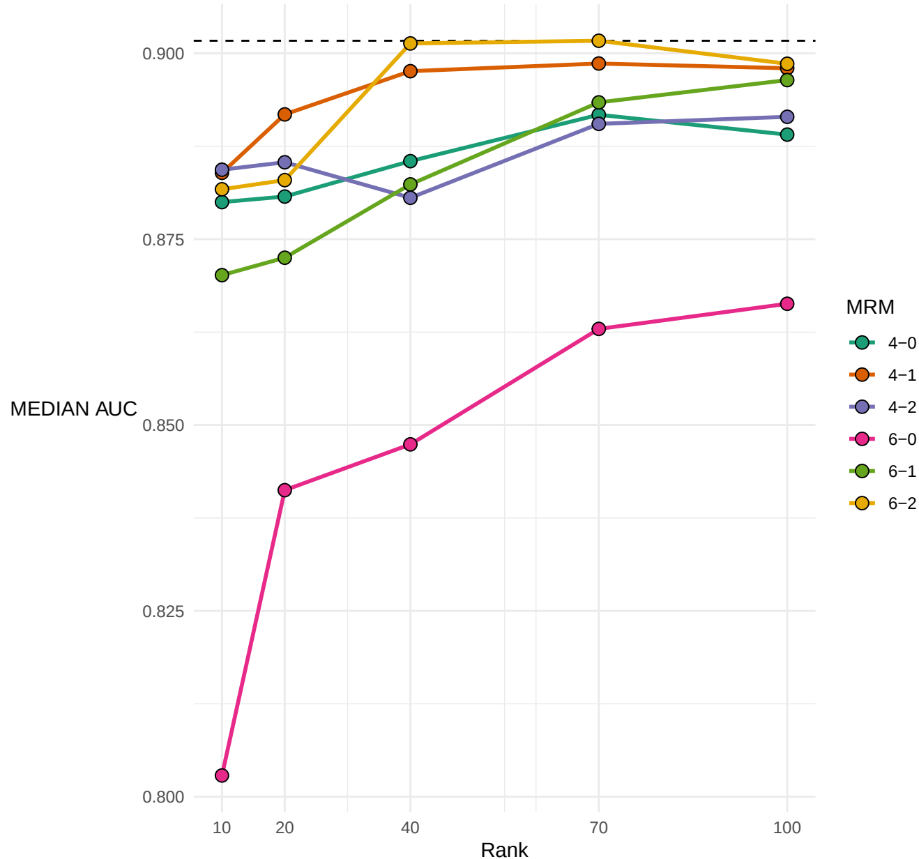
Median AUC across 23 optimiazion datasets for each Length~Gaps combination at each Rank
