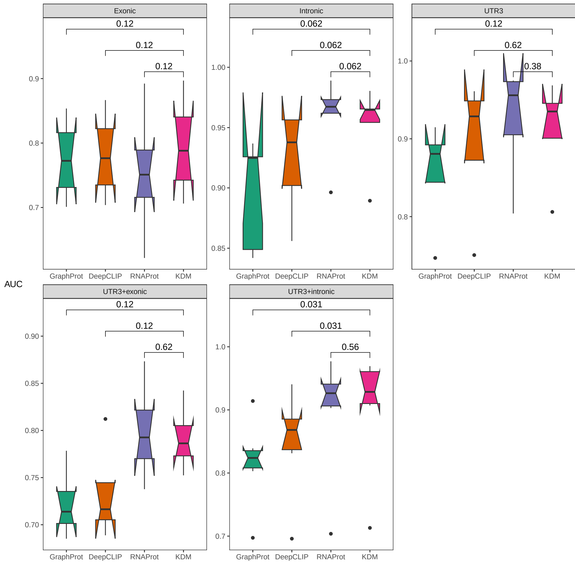
AUCs on RBP_24 with RNAProt datasets ~ Annovar Clusters
