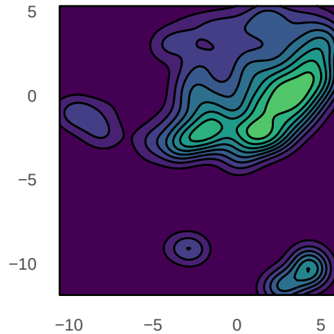
Active TSS (2070)
