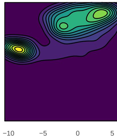
Enhancers (1439)
