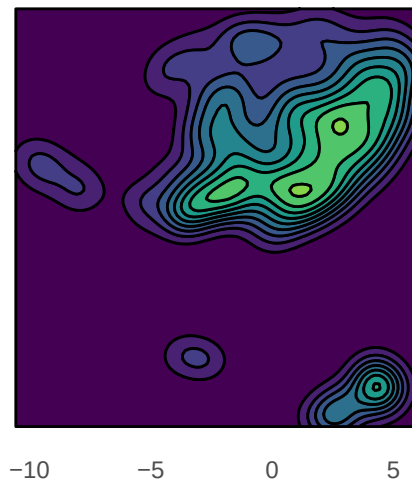
Bivalent/Poised TSS (2593)
